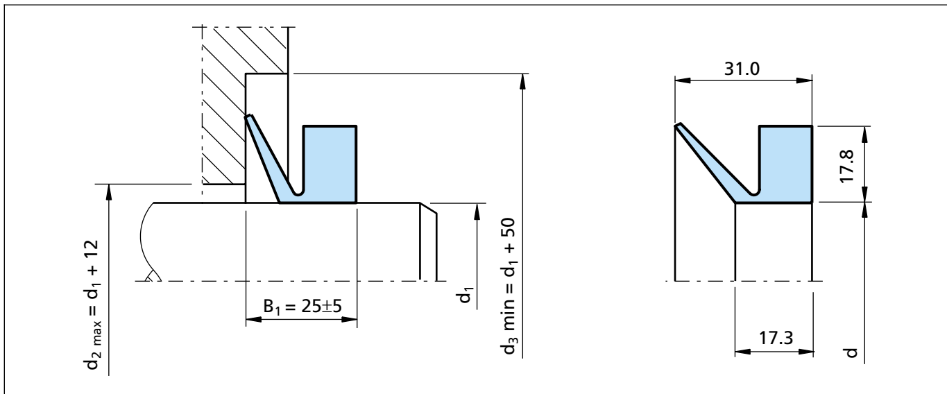
Figure 63 Installation drawing
