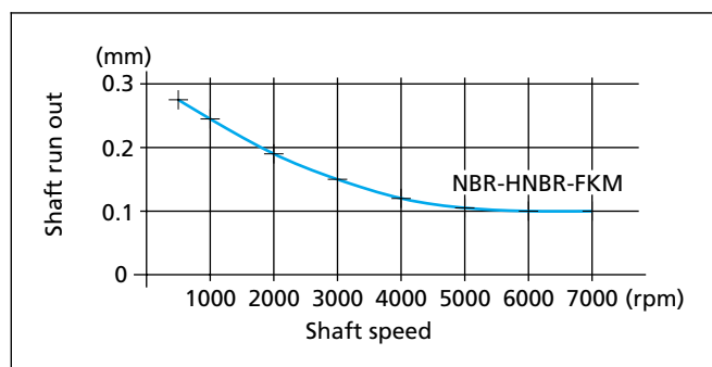
Figure 50 Permissible run out of the shaft
