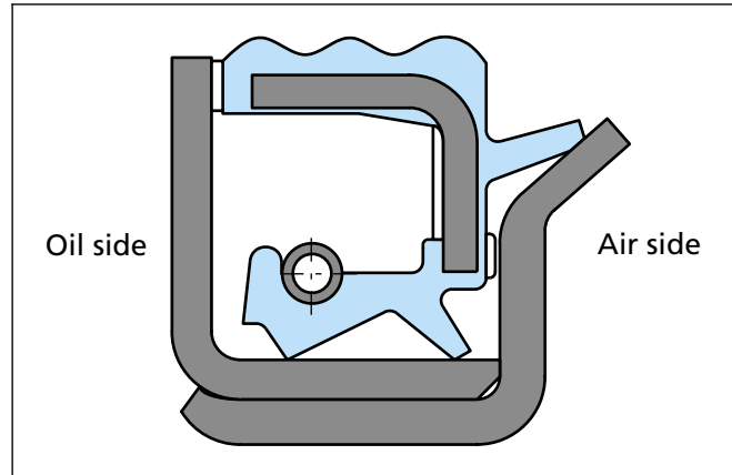
Figure 45 System 5000
