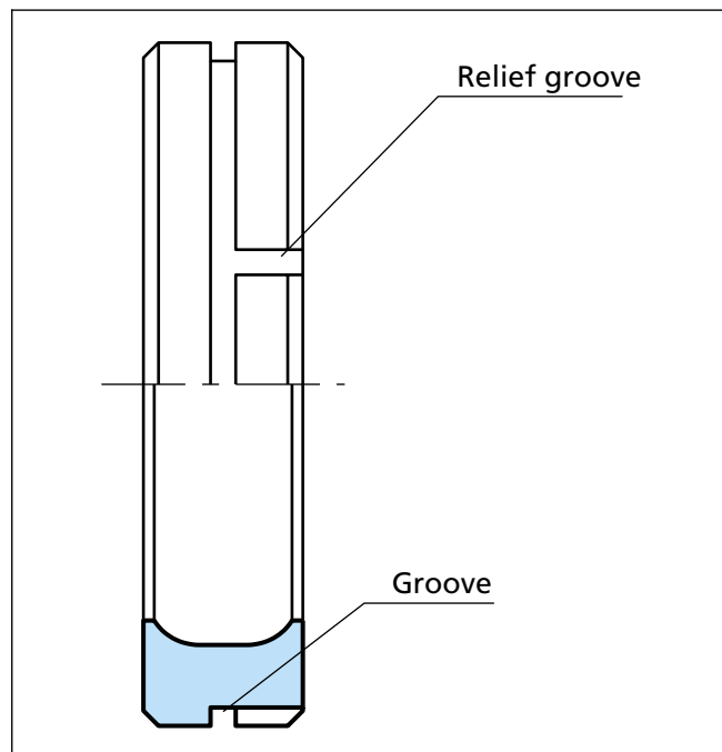
Figure 93 Turcon® Roto Glyd Ring® with pressure relief
