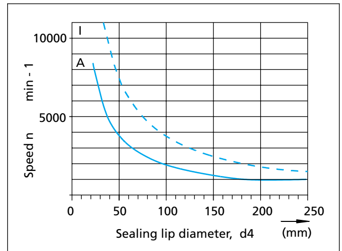
Figure 77 Maximum revolutions n as a function of sealing lip diameter d_4
