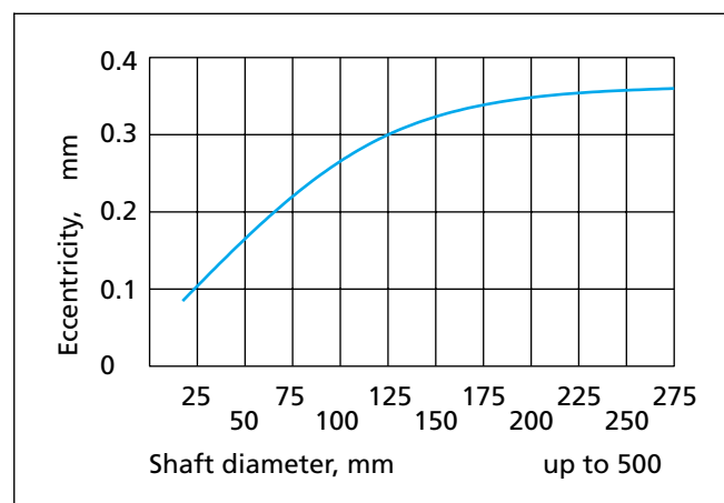
Figure 14 Eccentricity
