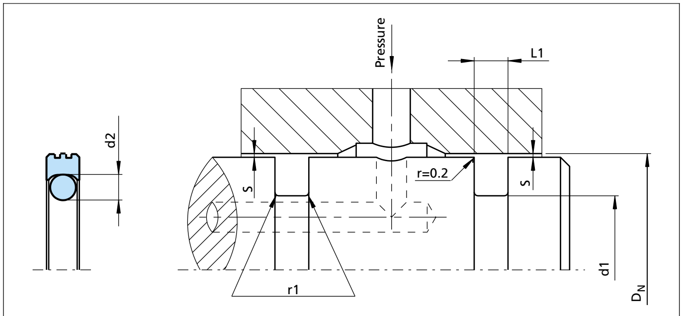
Figure 90 Installation drawing
