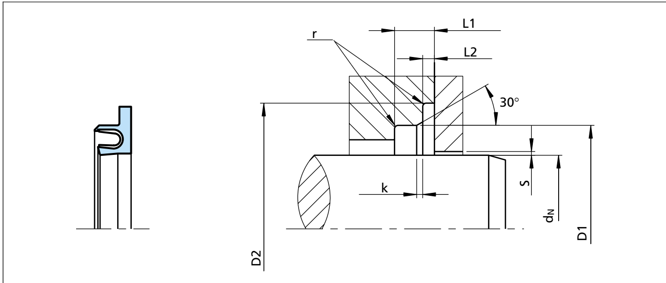
Figure 98 Installation drawing
