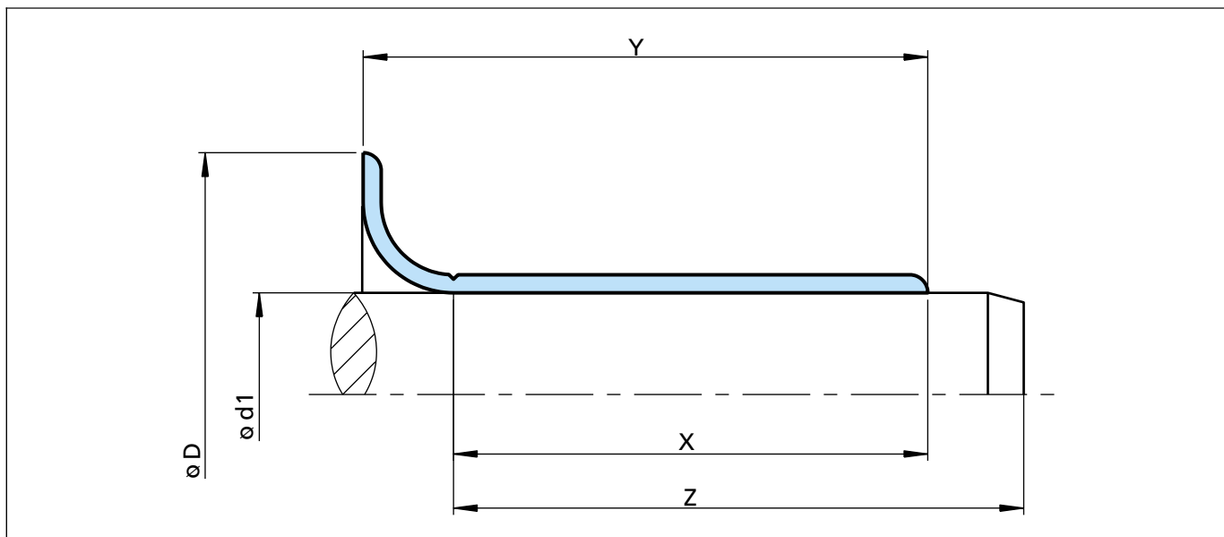
Figure 42 Installation drawing
