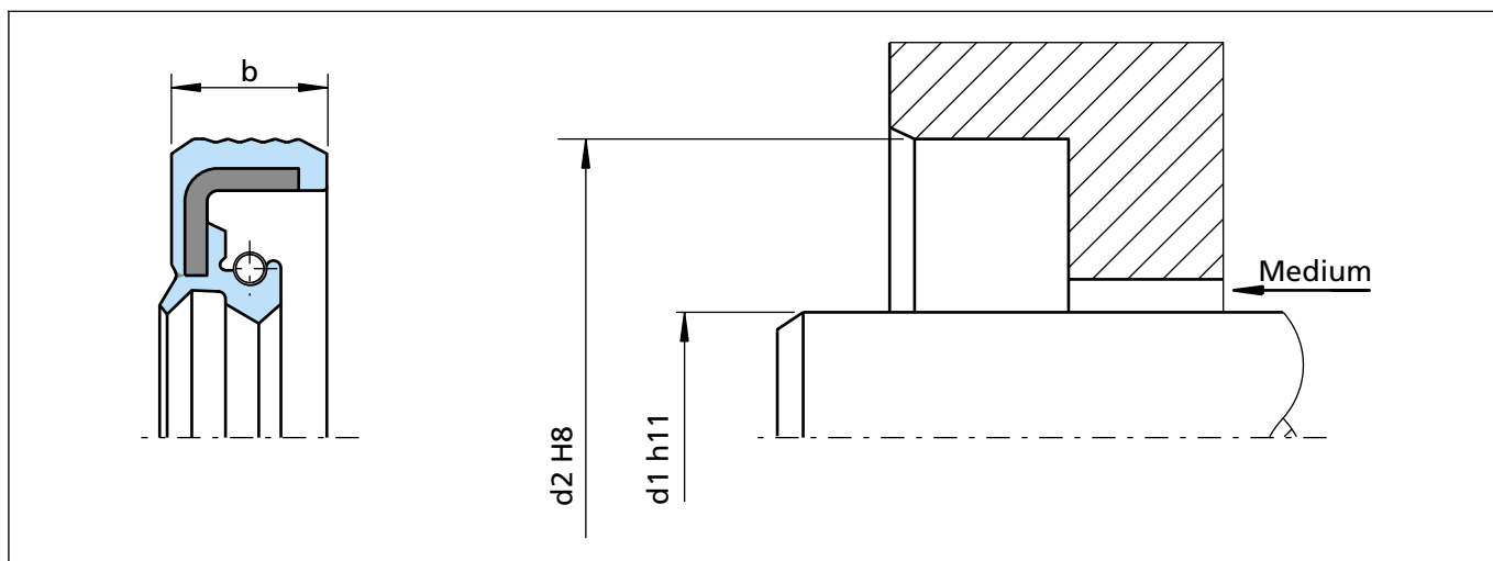
Figure 25 Installation drawing
