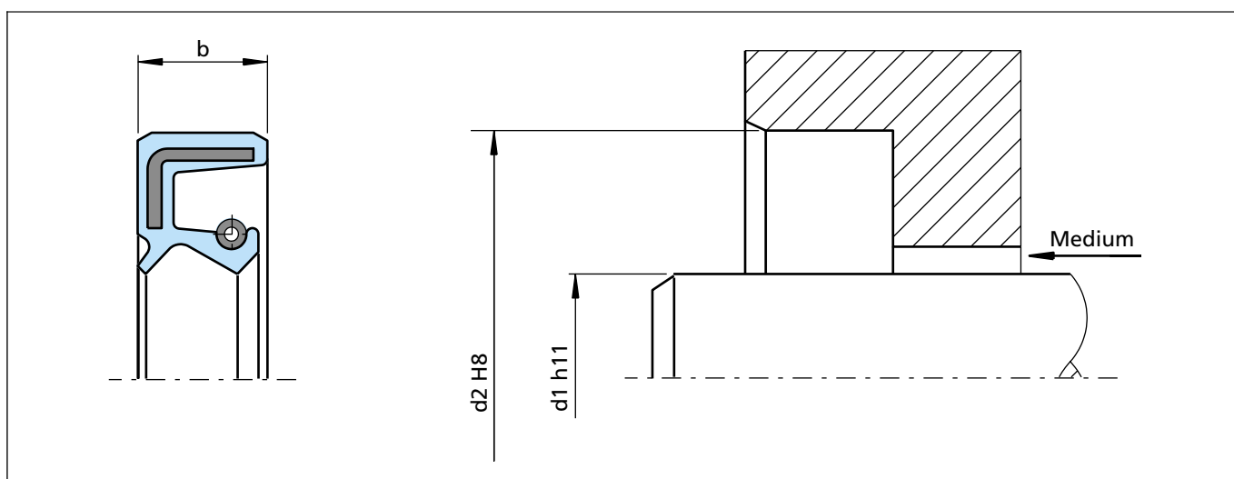
Figure 17 Installation drawing
