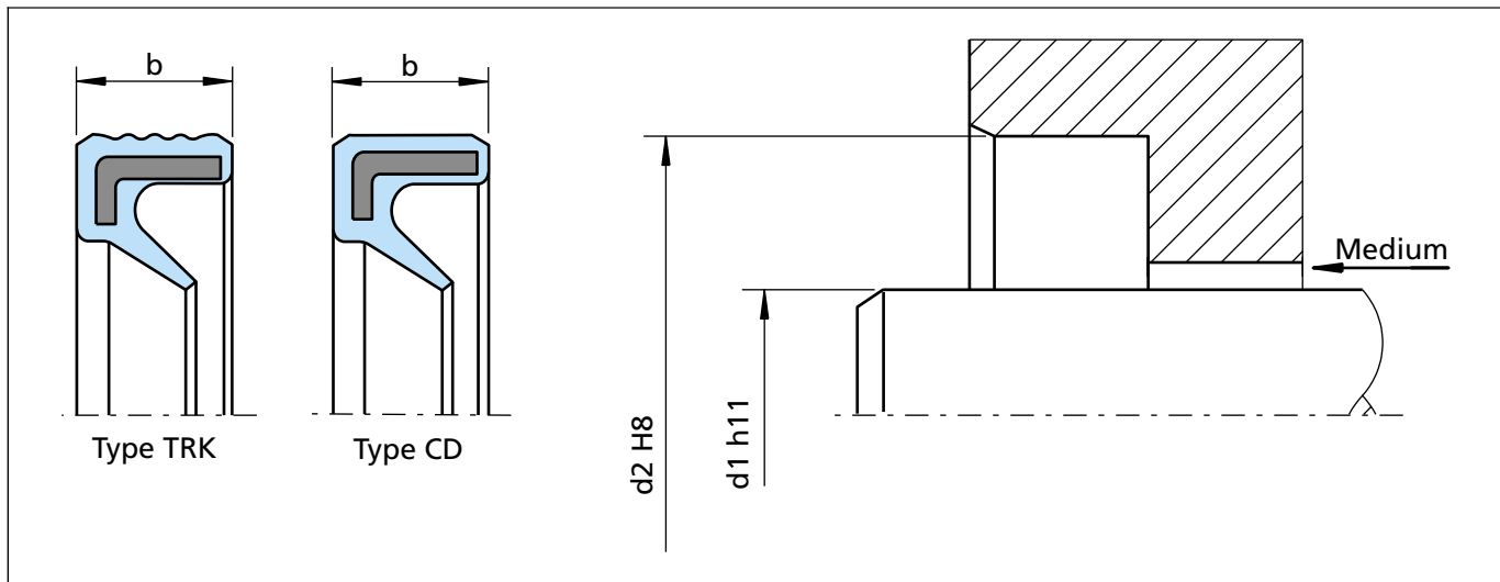
Figure 27 Installation drawing
