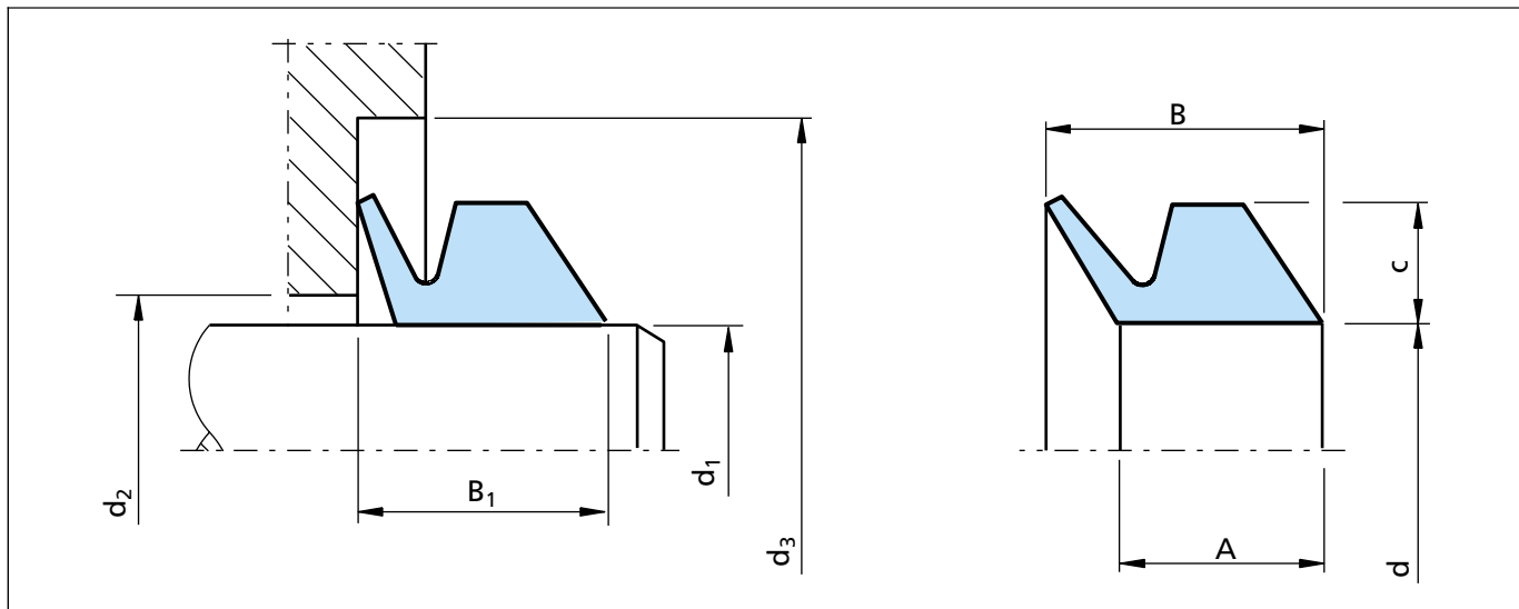
Figure 60 Installation drawing
