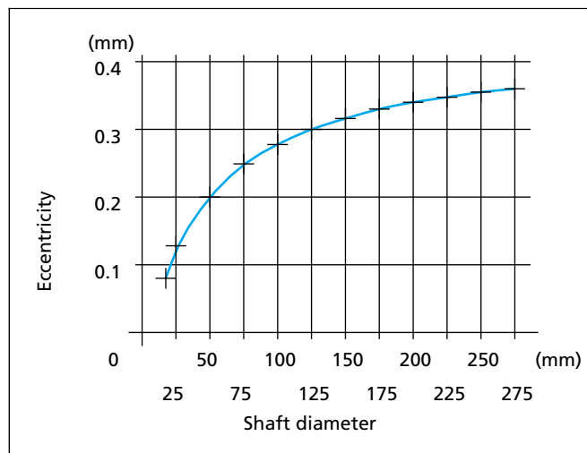
Figure 51 Permissible eccentricity
