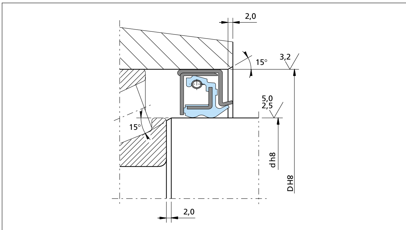
Figure 48 System 500 in wheel hub application
