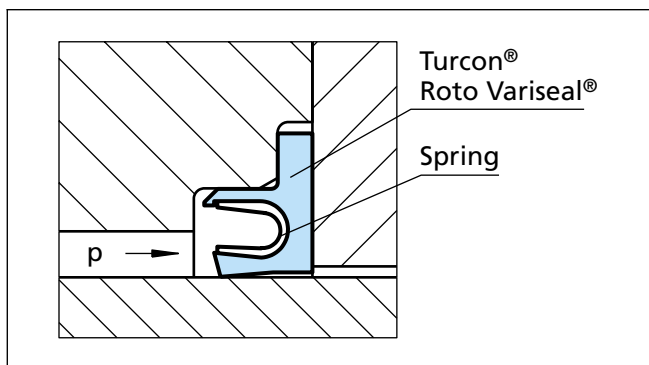
Figure 94 Turcon® Roto Variseal®
