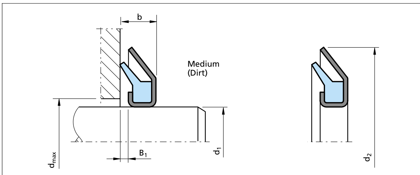
Figure 72 Installation drawing
