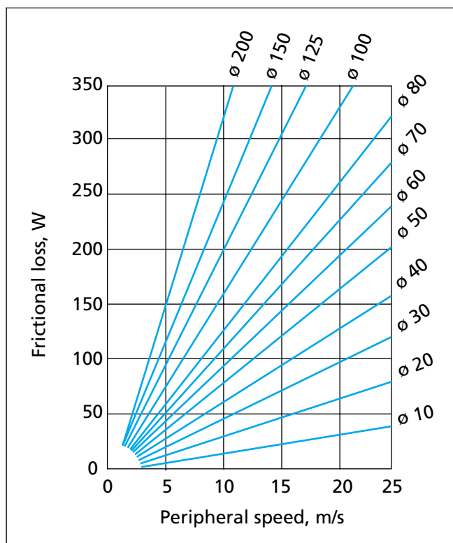
Figure 12 Frictional loss for TRA/CB type seal of nitrile rubber
