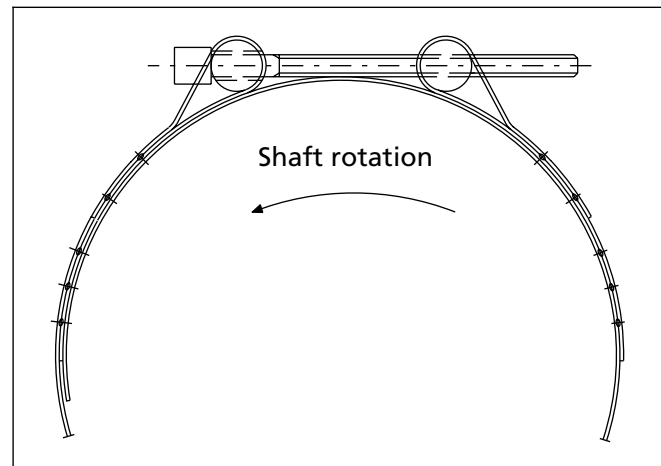
Figure 57 Clamping band RM
