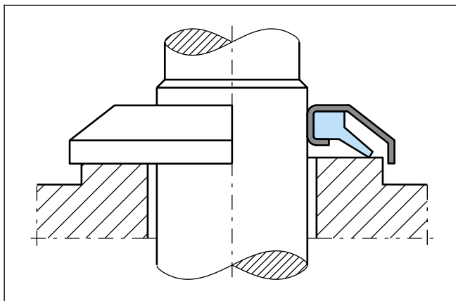
Figure 66 Vertical installation
