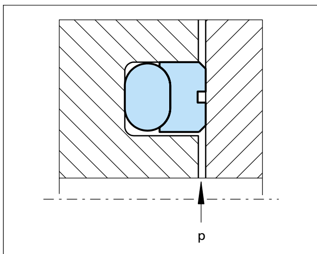
Figure 92 Axial acting Turcon® Roto Glyd Ring®
