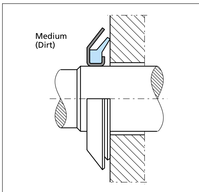
Figure 67 Installation drawing
