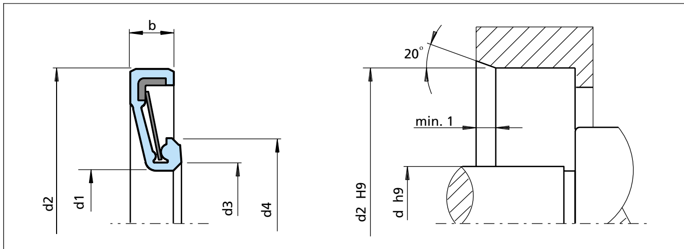
Figure 79 Installation drawing
