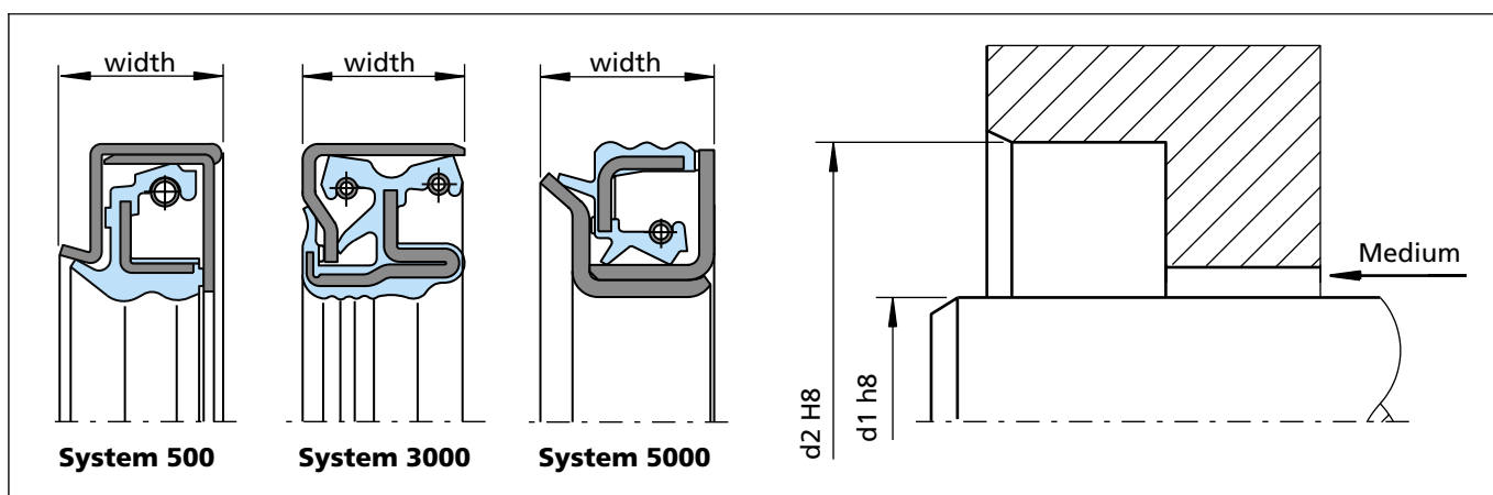
Figure 46 Installation drawing
