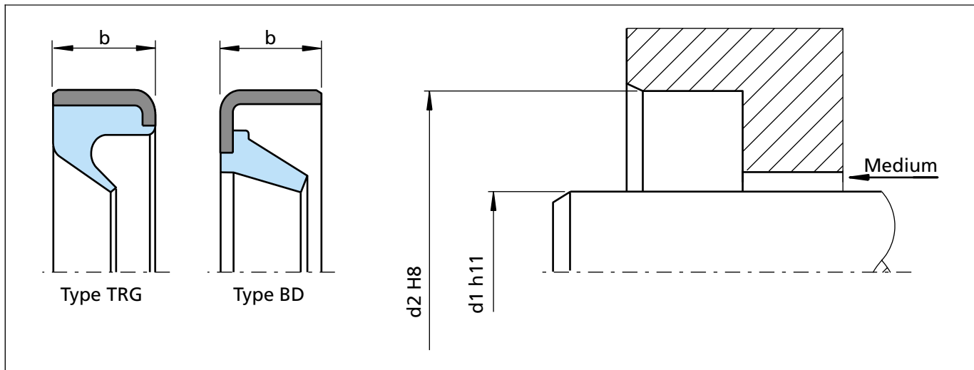
Figure 28 Installation drawing
