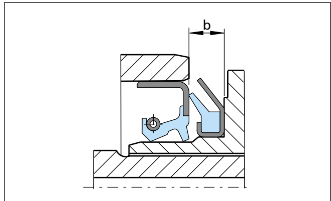
Figure 30 GAMMA seal fitted on the shaft boss
