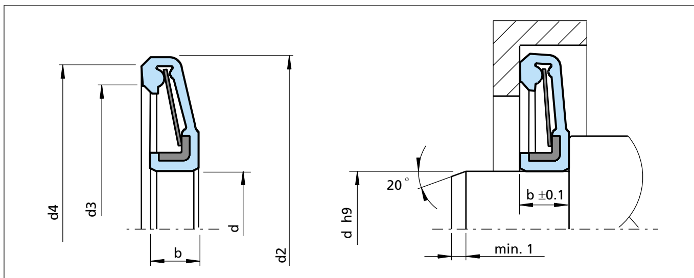
Figure 80 Installation drawing
