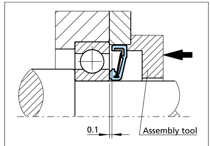
Figure 78 Installation of the axial shaft seal using an assembly tool.
