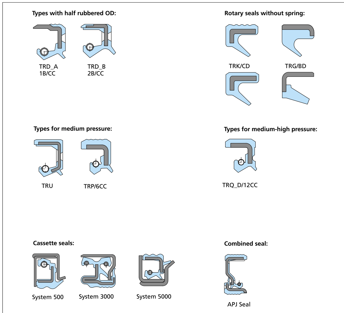
Figure 22 Selection of special radial seals
