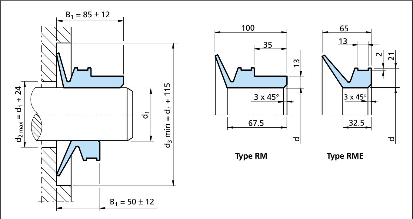
Figure 62 Installation drawing
