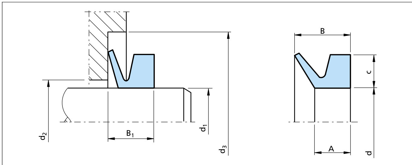
Figure 59 Installation drawing
