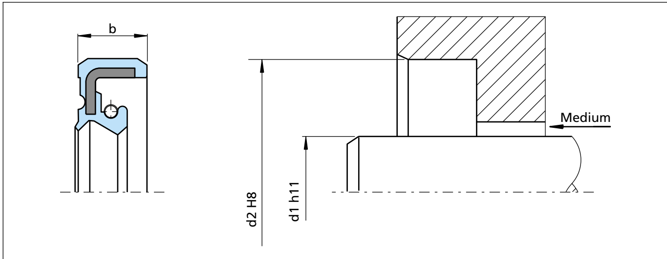
Figure 26 Installation drawing
